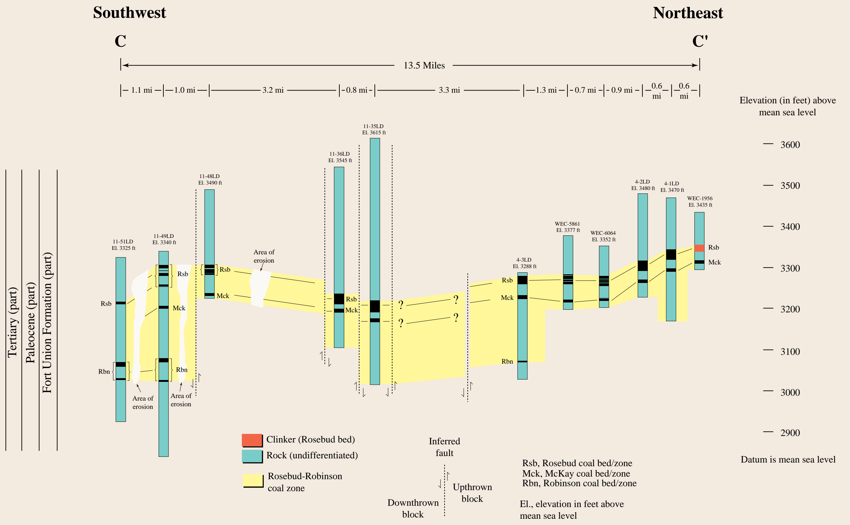
Figure PC-9. Southwest-Northeast cross section C-C', Colstrip coalfield, south-central Montana.
